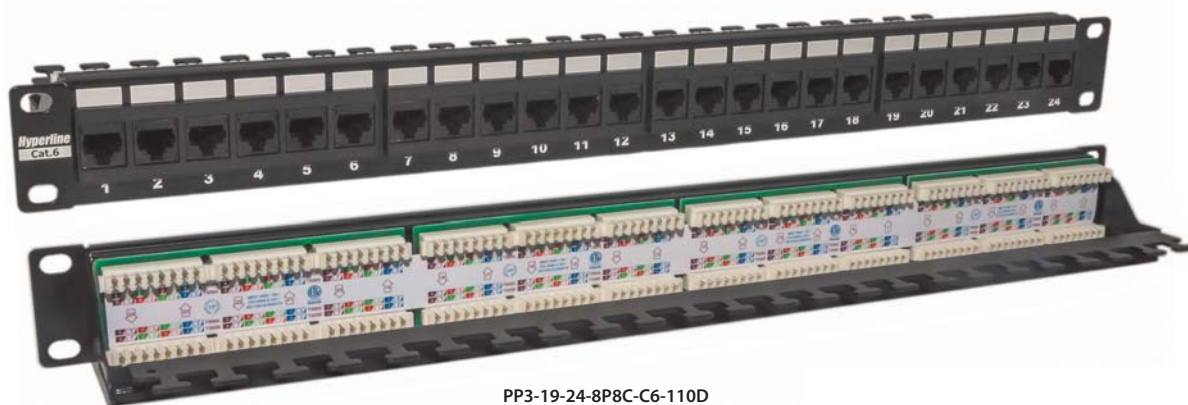
PP3-19-24-8P8C-C6-110D
